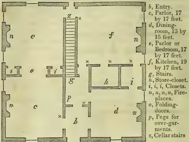
Fig. 29. Ground-floor.
